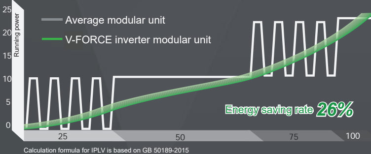
Energy Efficiency Curves of V-FORCE/Average Modular Units During Operation
